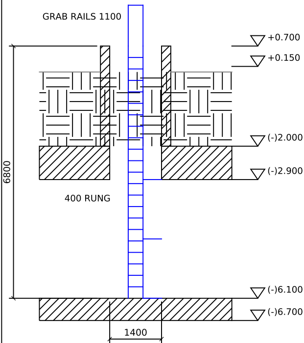
3 ESCAPE SHAFT - SECTION 1 : 100 ESC 1 AND ESC 2
