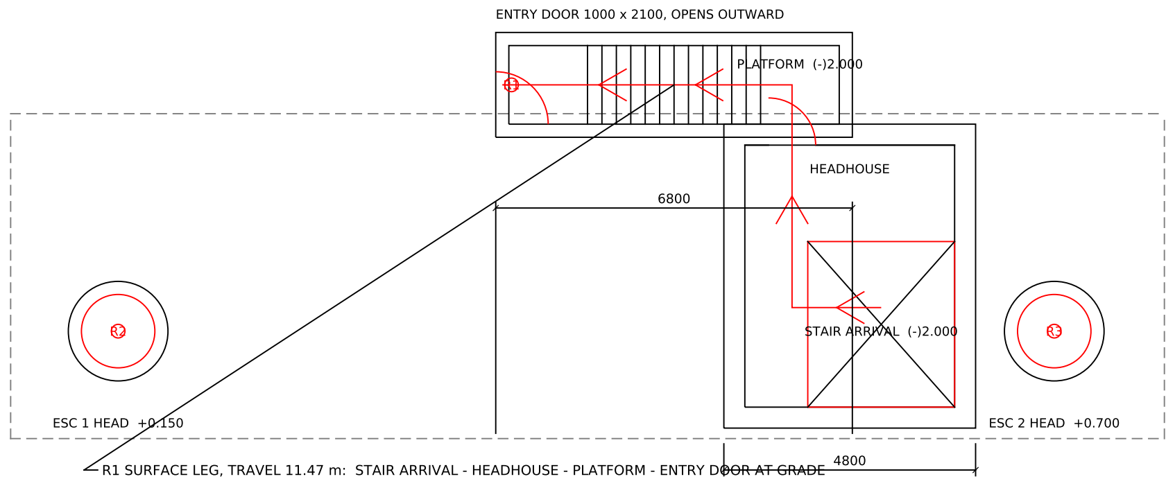
2 ENTRY LEVEL ESCAPE PLAN (-)2.000 AND 0.000 1 : 100 R1 EMERGES OUTSIDE THE PROTECTIVE BOUNDARY
